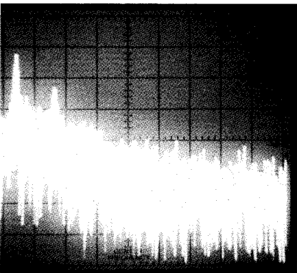
Fig 4—Spectral displays of the Yaesu FT-747GX transmitter output during composite-transmitted-noise testing. Power output: 100 W at 14 MHz (at A) and 100 W at 3.5 MHz (at B). Each vertical division is 10 dB; each horizontal division is 2 kHz. The scale on the spectrum analyzer on which these photos were taken is calibrated such that the log reference level (the top horizontal line on the scale in the photos) represents -60 dBc/Hz, and the baseline is -140 dBc/Hz. Composite noise levels between -60 and -140 dBc/Hz may be read directly from the photographs. The carrier, which would be off the left edge of the photographs, is not shown. The photographs show noise at frequencies 2 to 20 kHz offset from the carrier.
