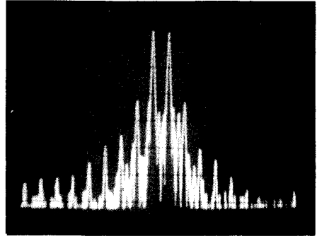
Fig 2—Spectral display of the Yaesu FT-747GX during two-tone intermodulation distortion (IMD) testing. Third-order products are approximately 32 dB below PEP output, and fifth-order products are approximately 45 dB down. Vertical divisions are each 10 dB; horizontal divisions are each 2 kHz. The transceiver was being operated at 100 W PEP output on 14.2 MHz.
