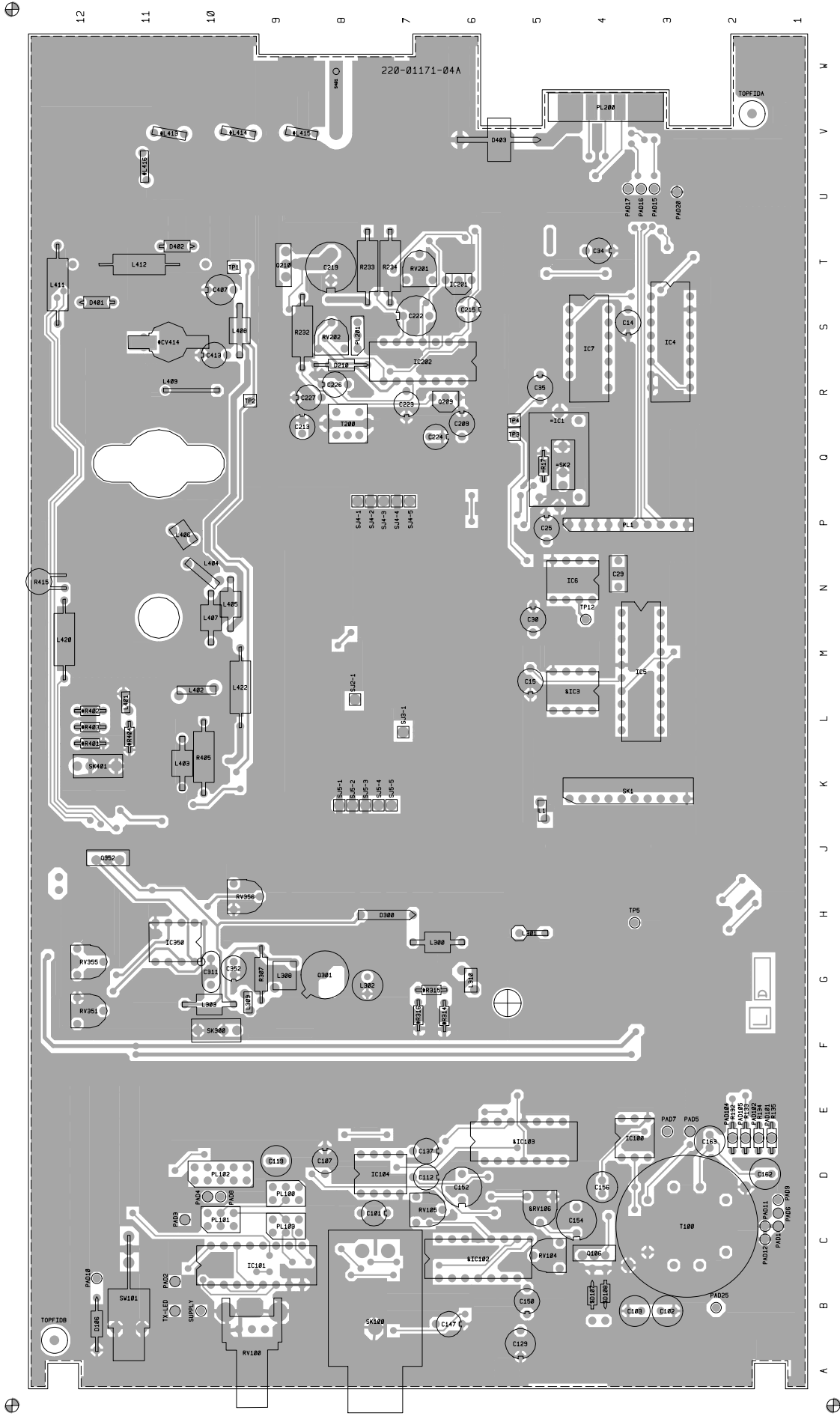
T866PCB Layout Top Side 220-01171-04
