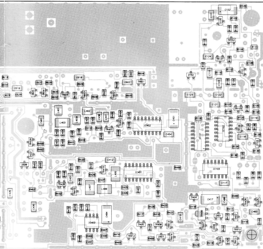
TX DRIVER ATO4881(VHF E Band) LAYOUT DIAGRAM
