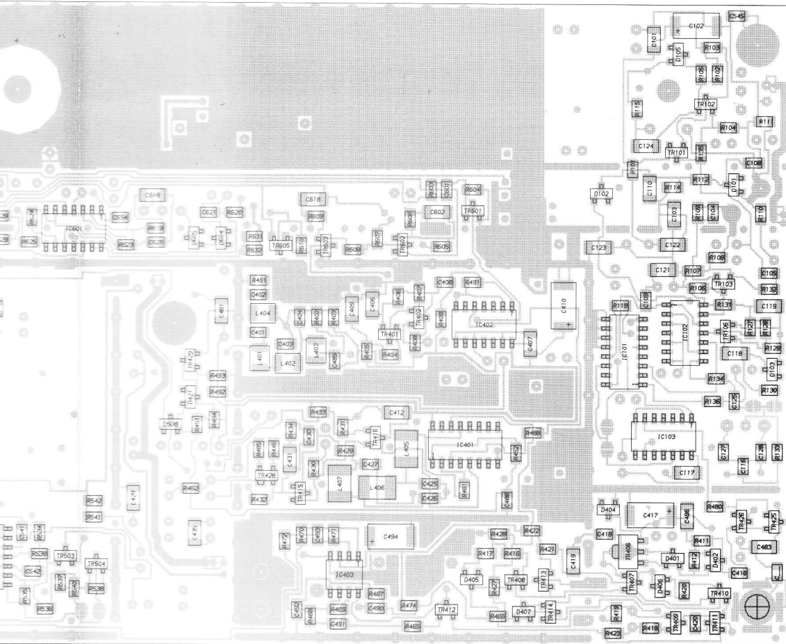
TX DRIVER ATO4881(VHF A & B Bands) LAYOUT DIAGRAM
