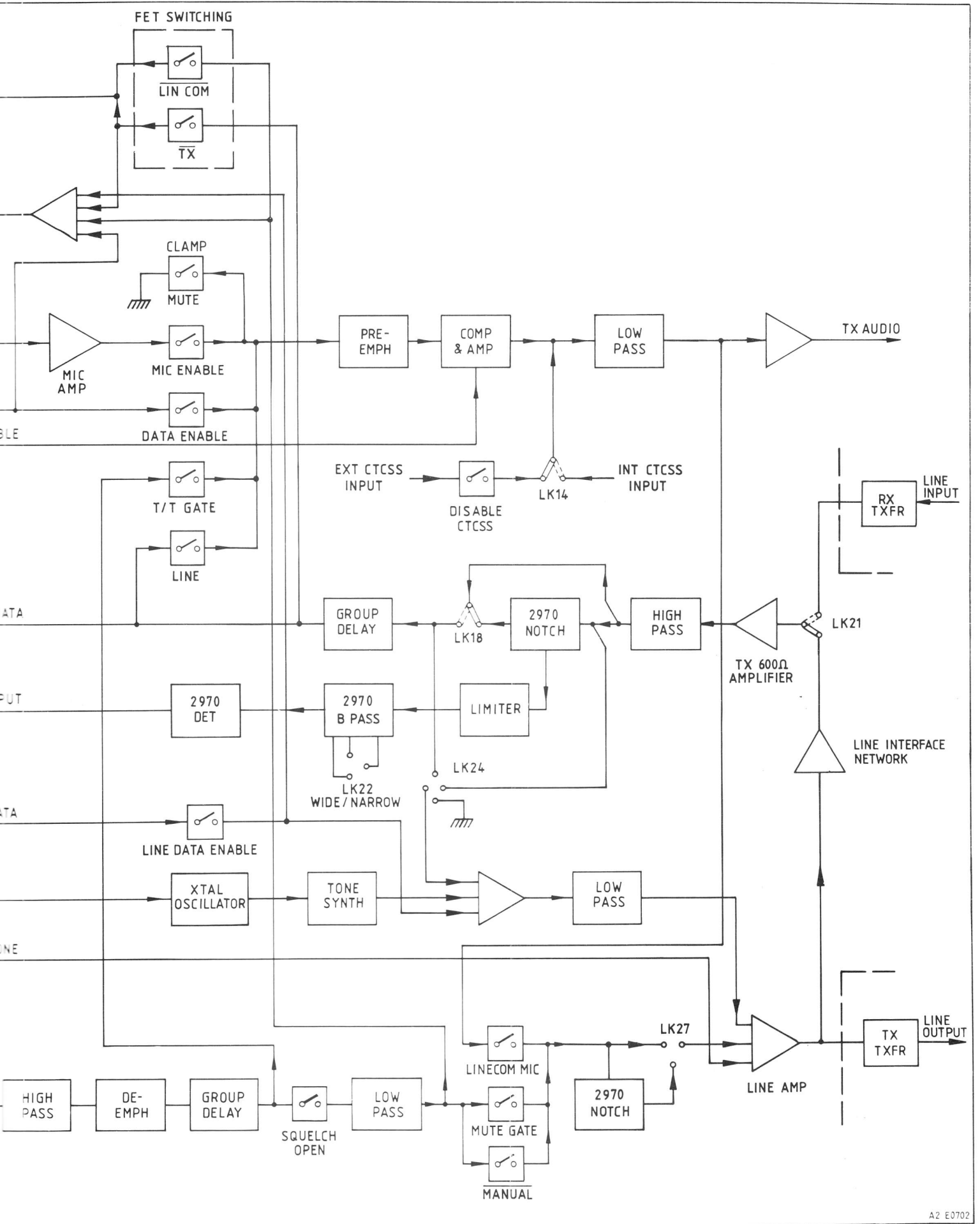
CONTROL MODULE ATO4872/- BLOCK DIAGRAM
