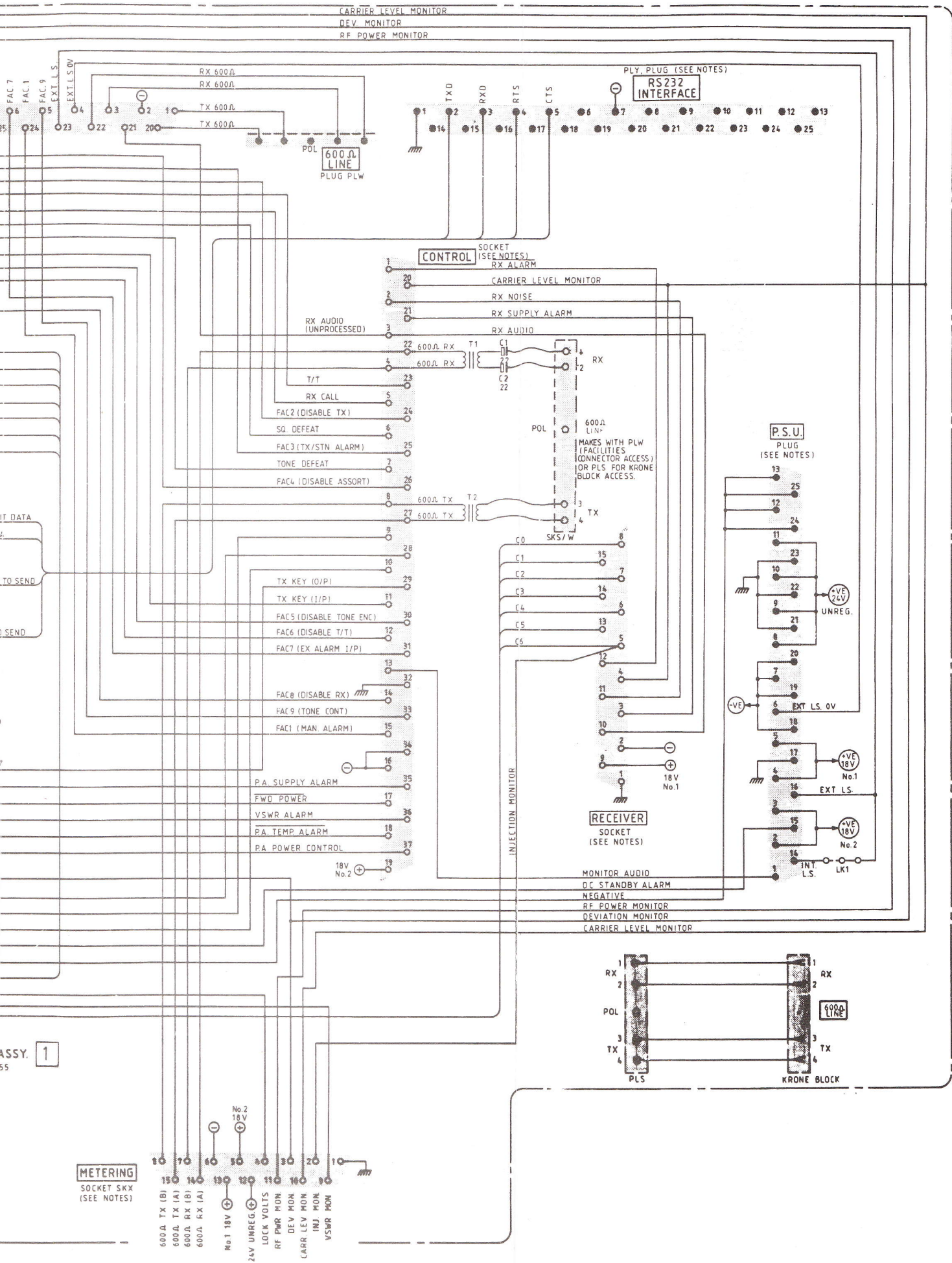
FIG. 4.2 BACKPLANE INTERCONNECTIONS
